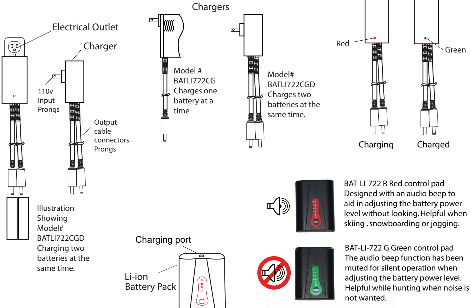
Figure 1. Lithium Battery and Chargers
